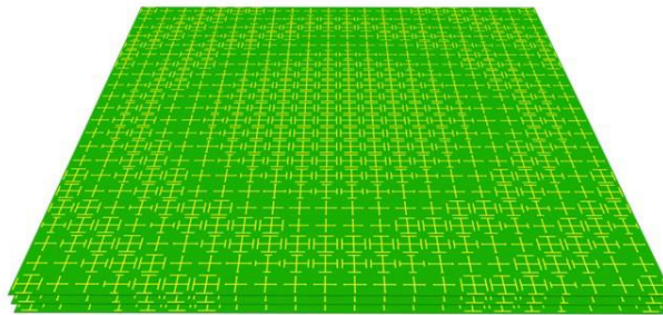
Metalens Antenna Using Conventional Jerusalem-Cross Metacells
