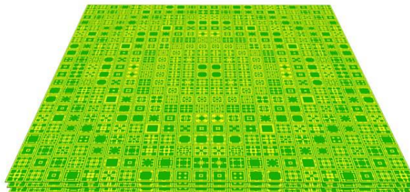
Metalens Antenna Using PK-DL Synthesized Metacells
